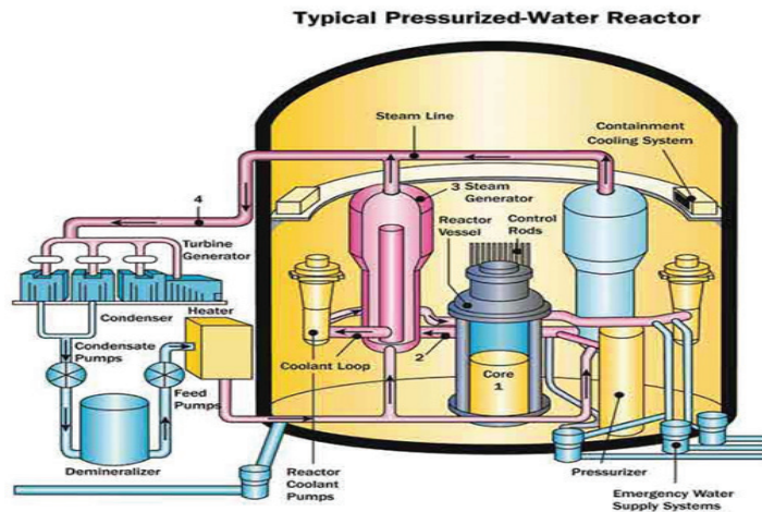
Figure 2. Pressurized Water Reactor
