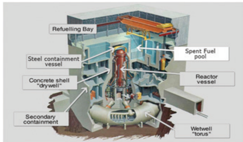
Figure 5. BWR Layout similar to Fukushima Daiichi
