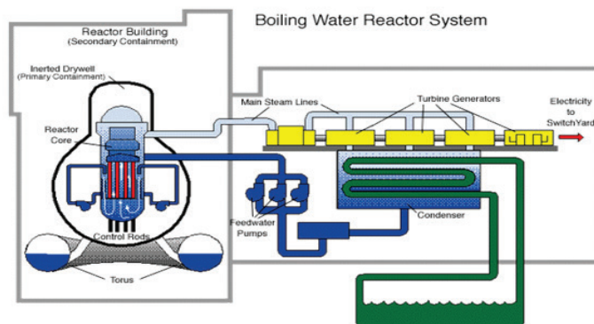
Figure 3. Boiling Water Reactor
