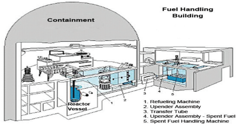
Figure 4. Typical PWR arrangement relative to Spent Fuel pool
